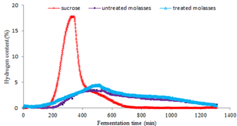
Figure 2. Hydrogen content of biogas produced by dark fermentation
