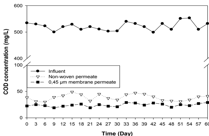
Figure 2: COD concentrations of influent, real and dynamic membrane Throughout MBR operation.
