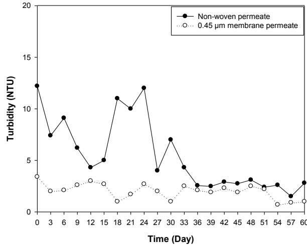
Figure 4: Turbidity results of dynamic and real membrane through MBR operation.
