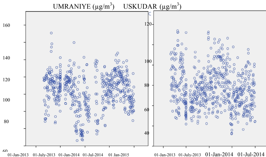
Figure 4. Nitrogen dioxide data
