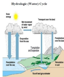
Figure 3: Hydrologic Cycle [11]
