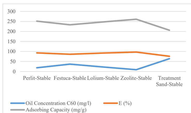
Figure 2. Yakakent Fisherman's Shelter Oil Concentration, Oil Removal Efficiency and Adsorbing Capacity ( C_{60}=60 \text{ min.} , adsorbent 0,1 g. C_0 = 270 \text{ mg/l} ).
