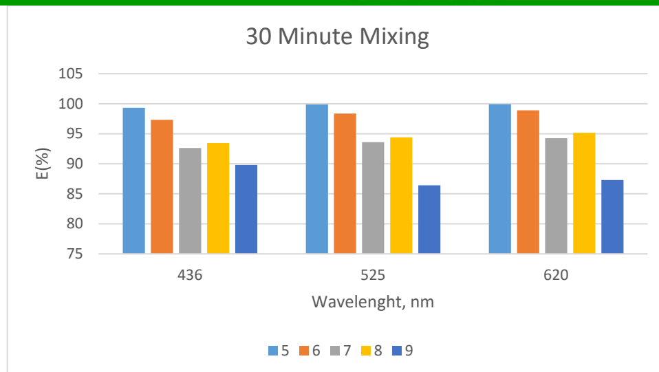
Figure 4. Color removal efficiencies at 30-minute mixing time
