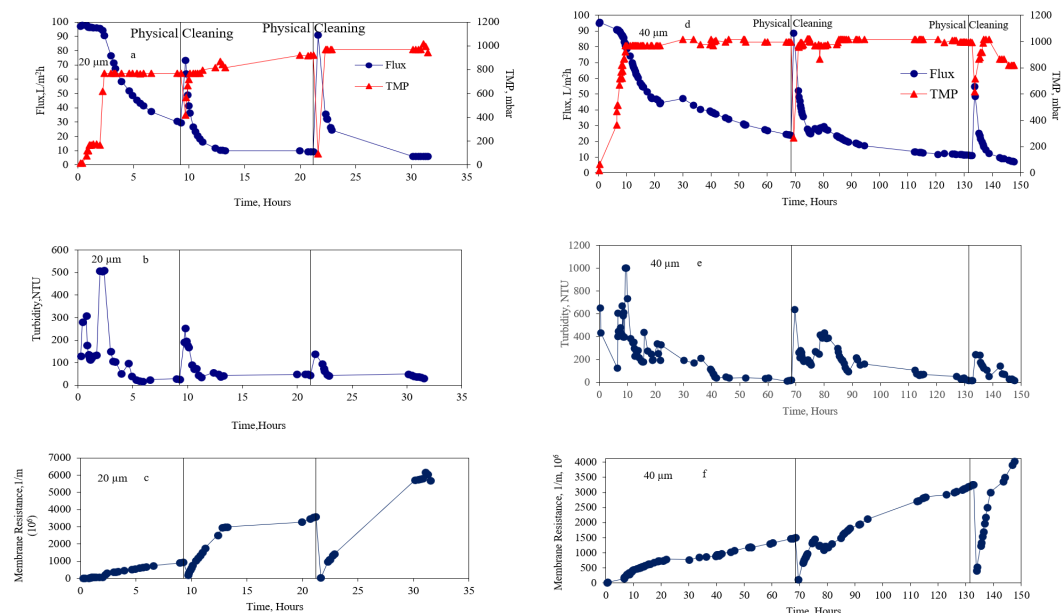
Figure 2. Change of (a) Flux and TMP, (b) Turbidity and (c) Membrane Resistance versus time at support material with 20 \mu\text{m} and Change of (d) Flux and TMP, (e) Turbidity and (f) Membrane Resistance versus time at support material with 40 \mu\text{m}
