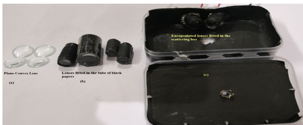
Figure 7. Image of (a) Plano-convex lens (b) Lenses fitted in the paper tube (c) Lenses encapsulated in a scattering box
