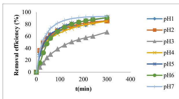
Figure 2. Removal efficiency (%) - t(\text{min}) graph for each pH
