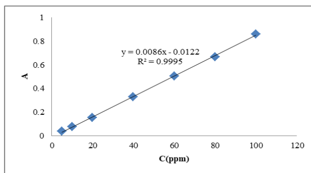
Figure 1. Calibration graph of Reactive Blue 28 dye
