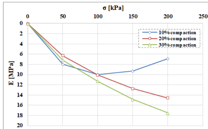
Figure 4. Compression modulus of foam glass aggregate for different amount of loads.
